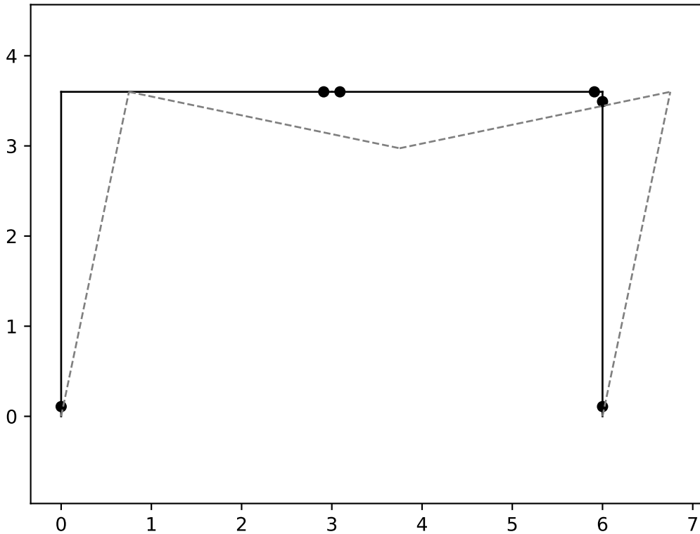
Plastic Mechanism ( \mathbf{F}_u = \lambda \cdot \mathbf{F}_{ref} with \lambda = 0.62500 \cdot M_u )
